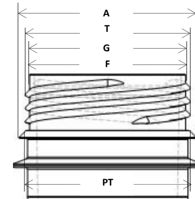
Rosca 48/40
